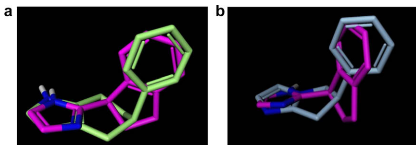
Figure 3. In silico overlap of (a) axial conformations of 5 (green) with 3 (purple) and (b) low energy conformation of 6 (blue) with 3 (purple).
